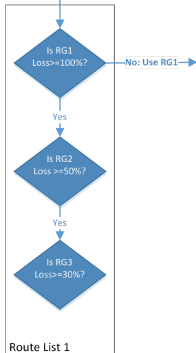
Figure 37 - Congestion-Aware Route List Logic
