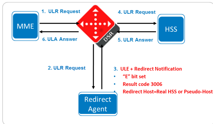
Figure 14 - Redirect Agent
