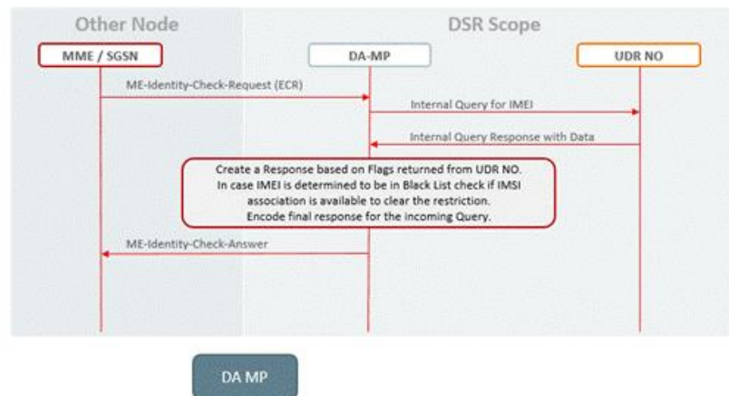
Figure 79 – S13 EIR Call Flow
