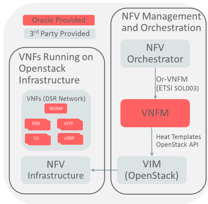
Figure 69 – DSR VNFM
