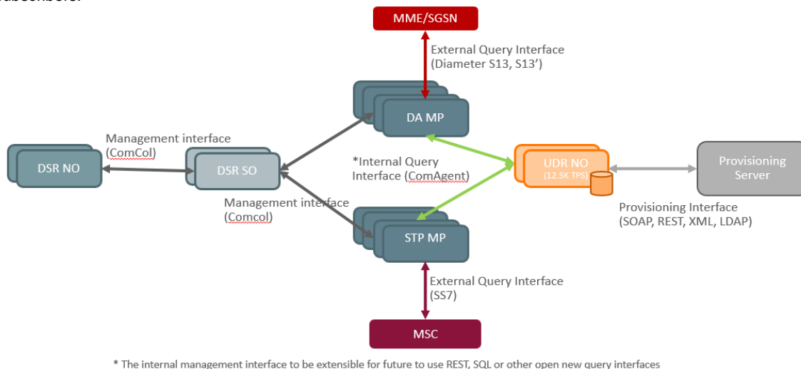
Figure 77 – EIR solution architecture.
