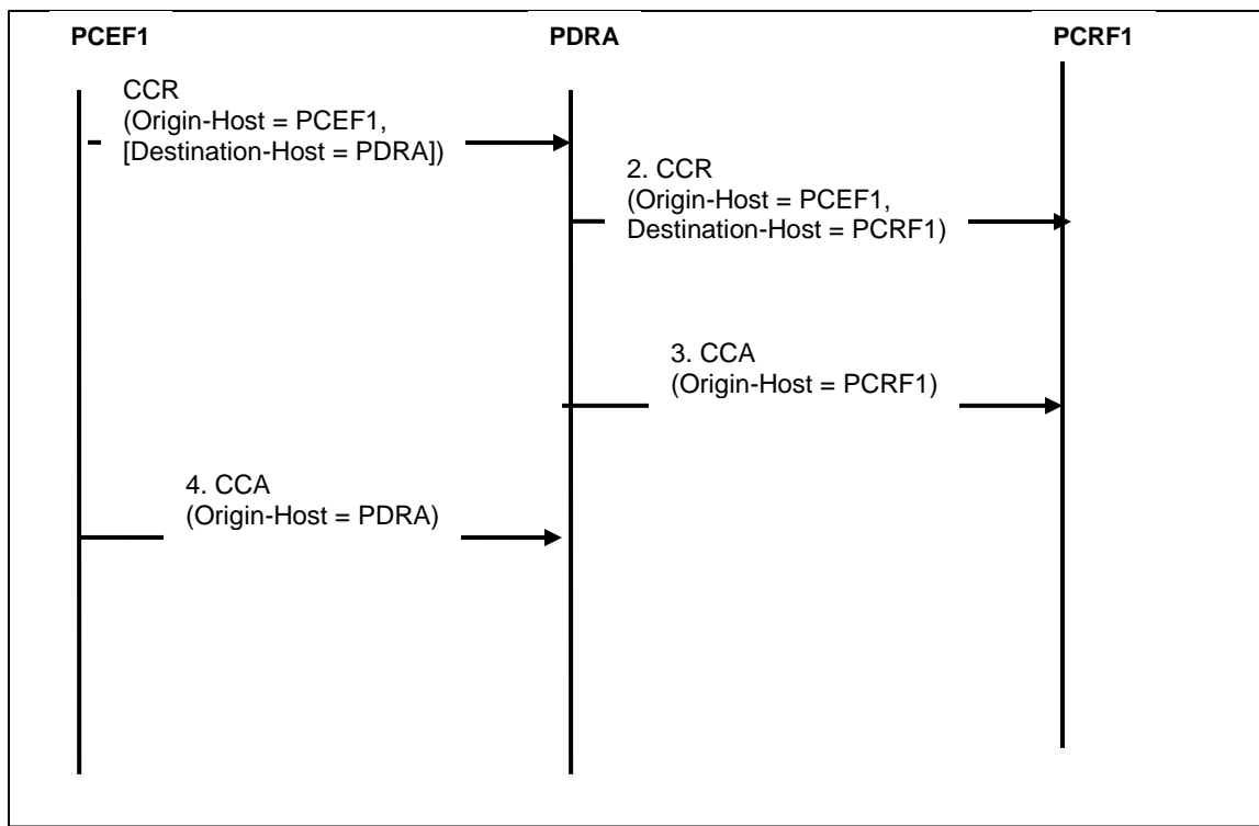
Figure 60 - PCR topology hiding
