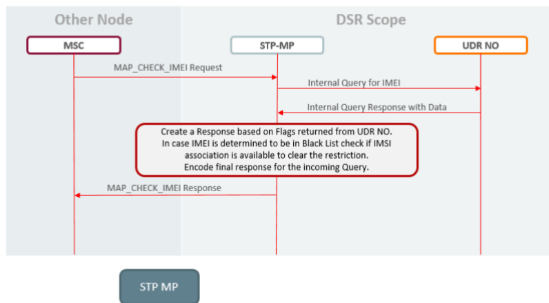
Figure 78 – SS7 EIR call flow
